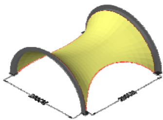
Fig. 5: Design for a double-curved shell.
