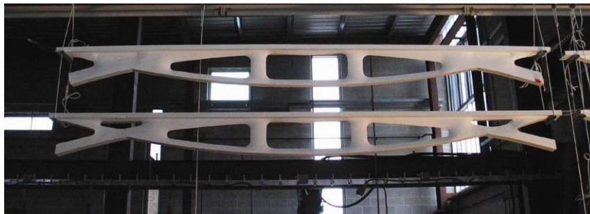
Fig. 1: Plaster models of lightweight trusses made with fabric formwork (West 2006).
