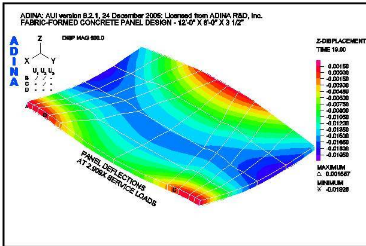
Fig. 13. Panel deflections.
