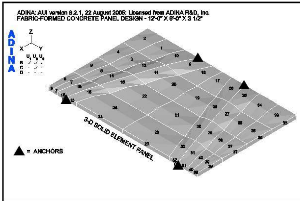
Fig. 12. Panel model.
