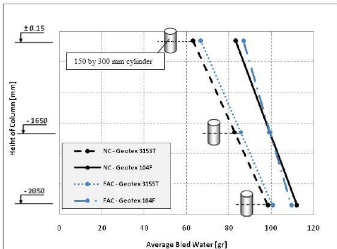
Figure 30: Average water loss through fabric formed cylinders.
